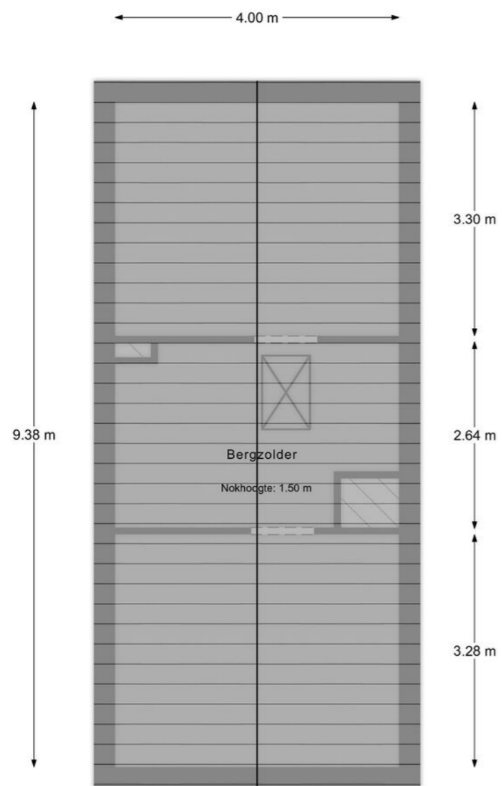
Bergzolder
